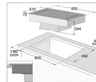
IN APPOGGIO - SURFACE MOUNTED
