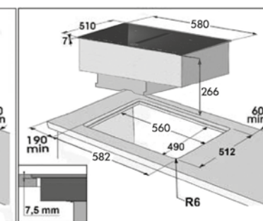
A FILO - FLUSH MOUNTED
