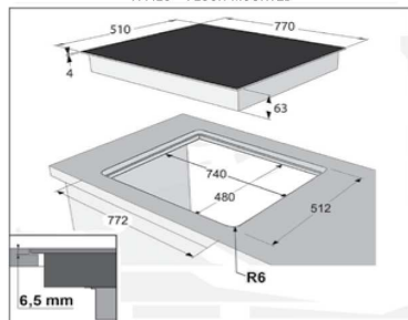
A FILO - FLUSH MOUNTED
