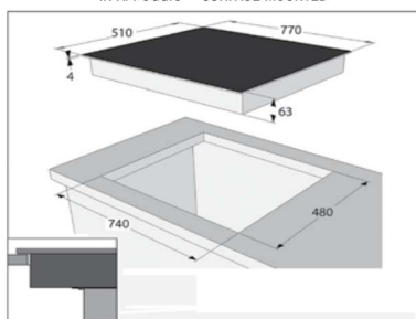
IN APPOGGIO - SURFACE MOUNTED
